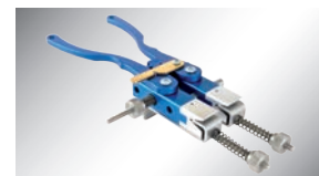
GUIDING CLAMPS FZ01 VARIO with exchangeable profile jaws, for round belts with diameters of up to 10 mm and V-belt profiles up to 10 (Z)
