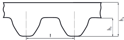
Principle sketch
